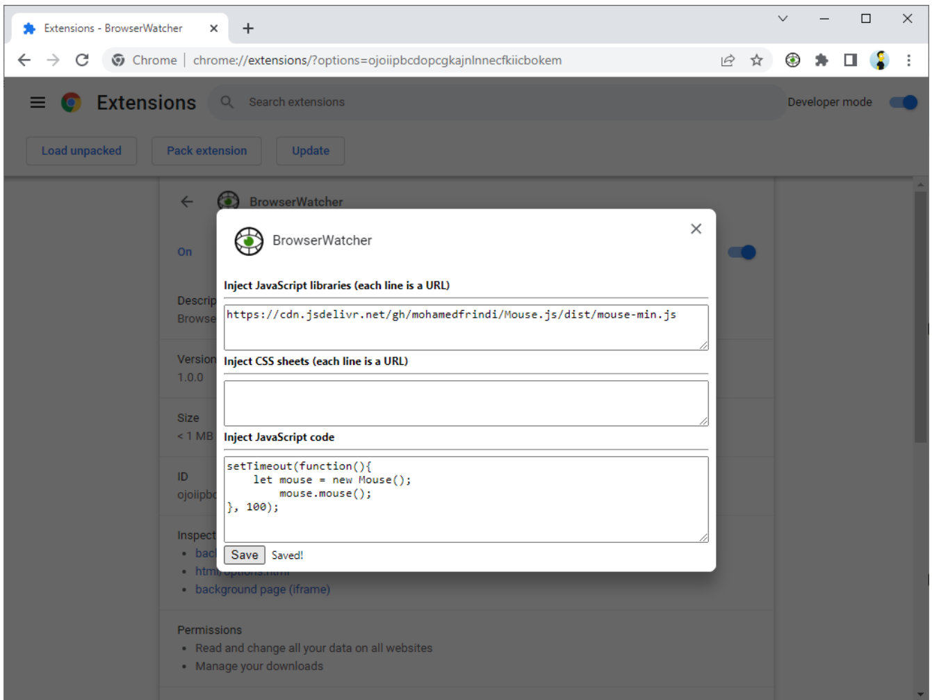
Figure 9. BrowserWatcher options page (example for highlighting mouse)
